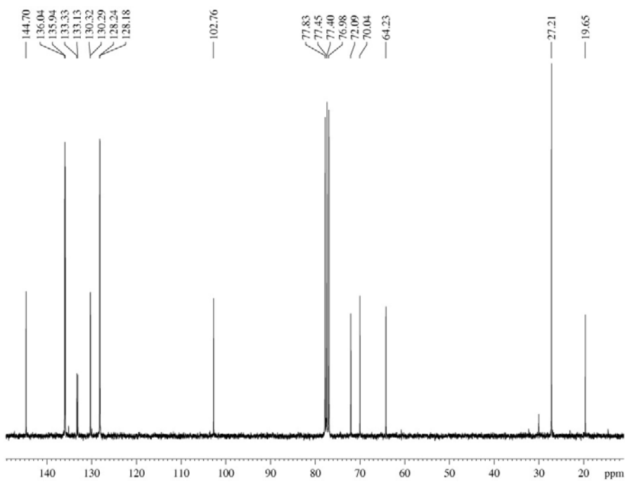
1 H and 13 C spectra of compound 13
