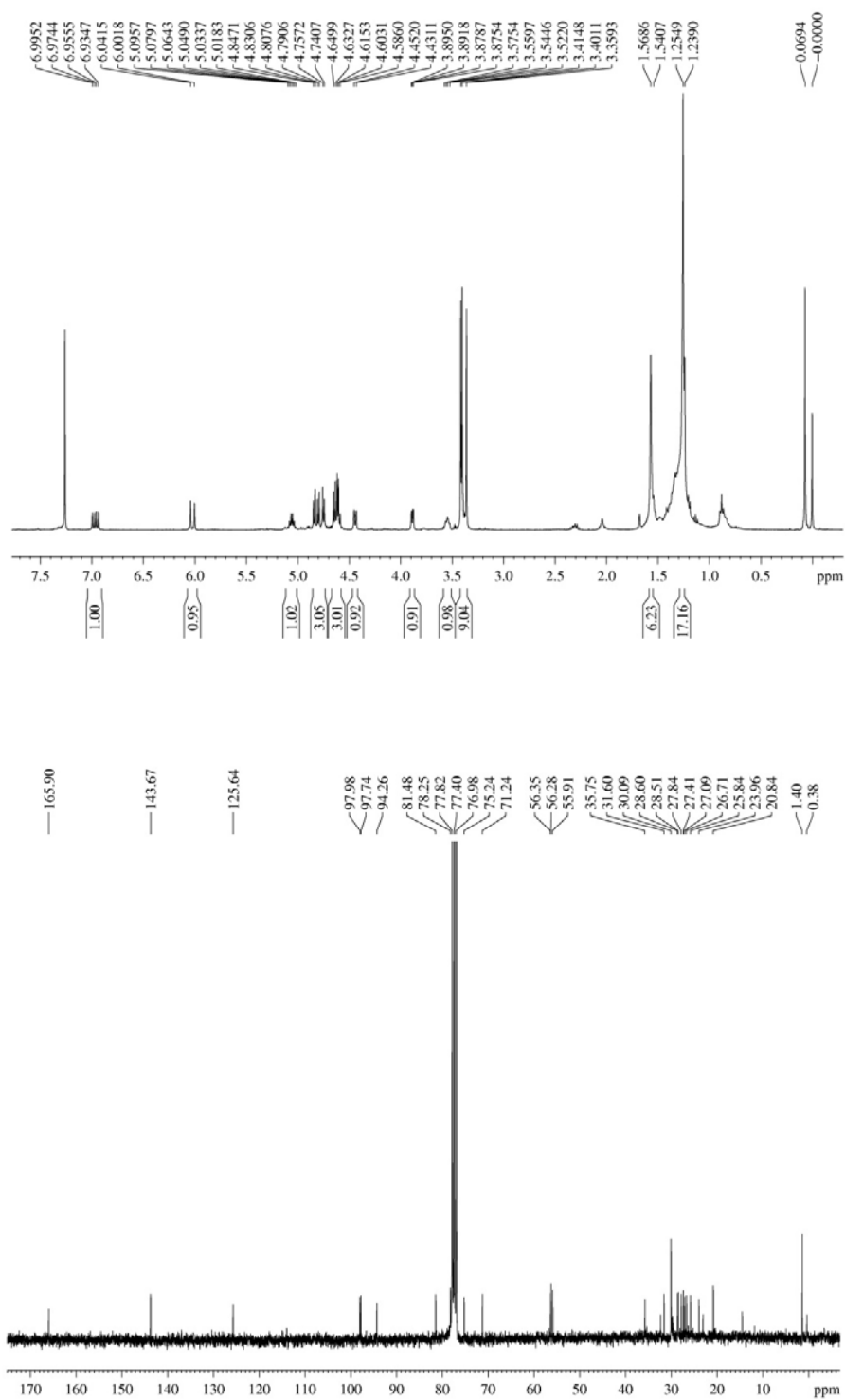
^1\text{H} and ^{13}\text{C} spectra of compound 18
