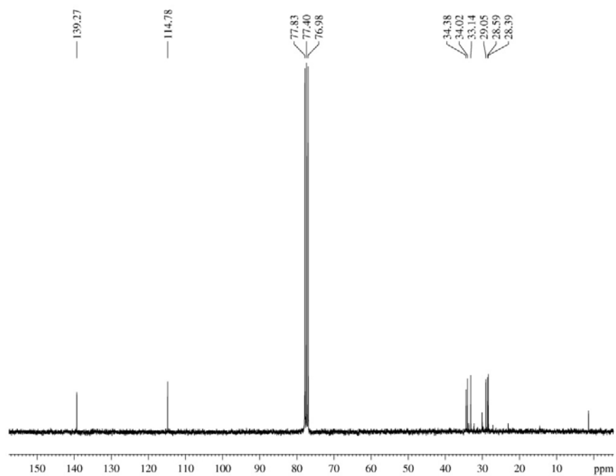
1 H and 13 C spectra of compound 10
