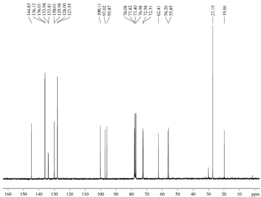
1 H and 13 C spectra of compound 14
