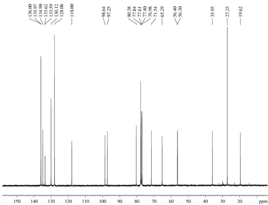
1 H and 13 C spectra of compound 15
