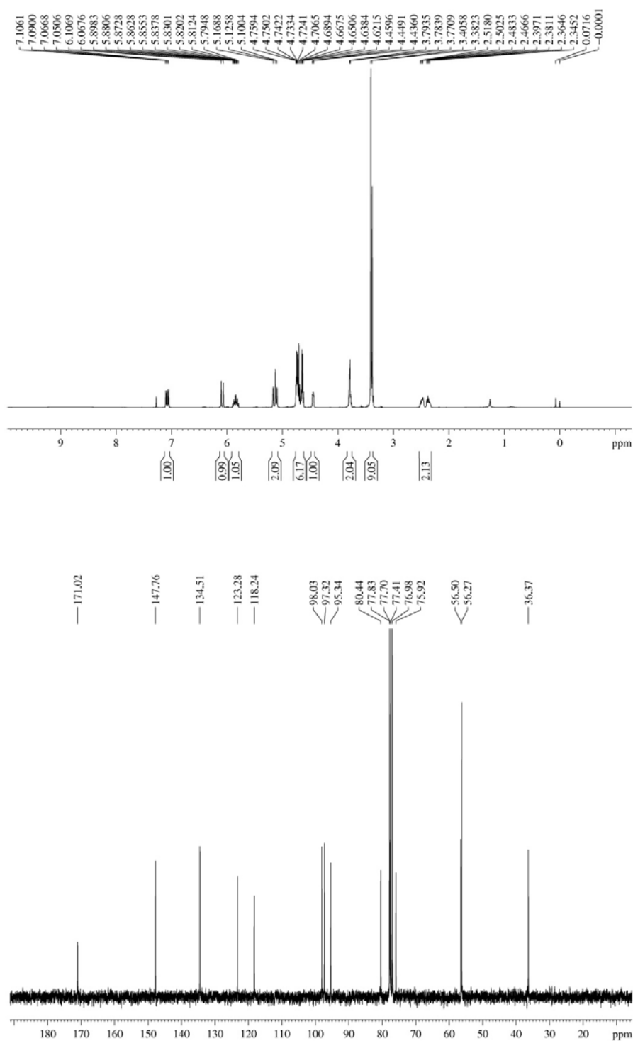
^1\text{H} and ^{13}\text{C} spectra of compound 5
