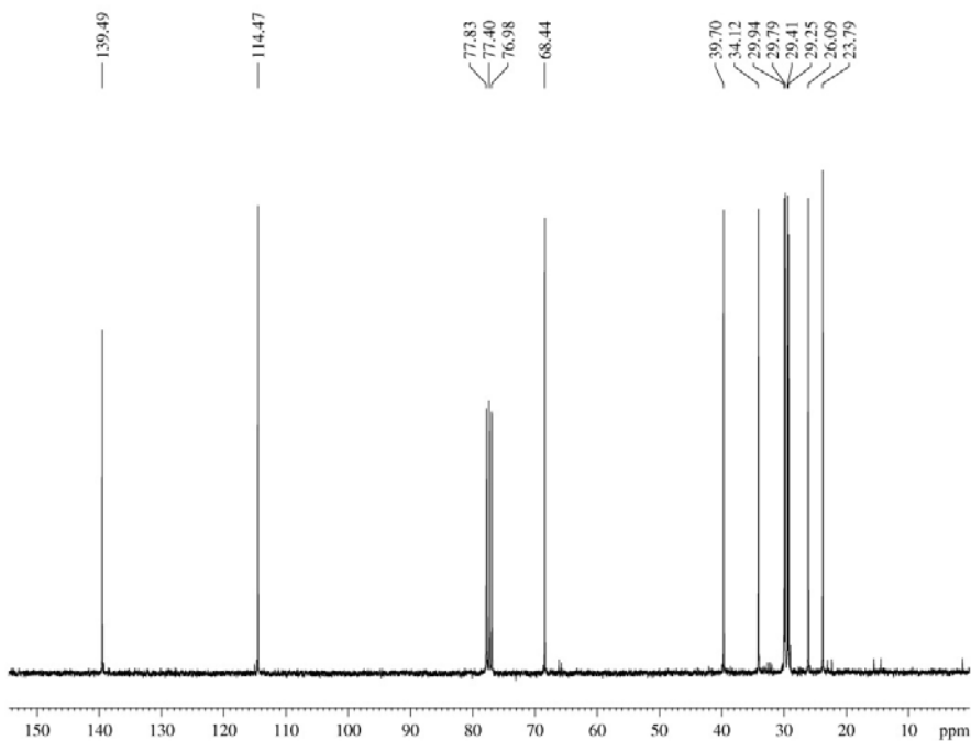
^1\text{H} and ^{13}\text{C} spectra of compound 6
