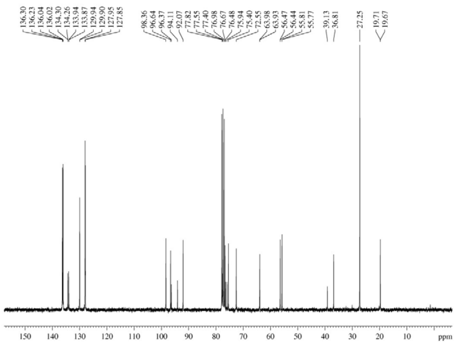
1 H and 13 C spectra of compound 9
