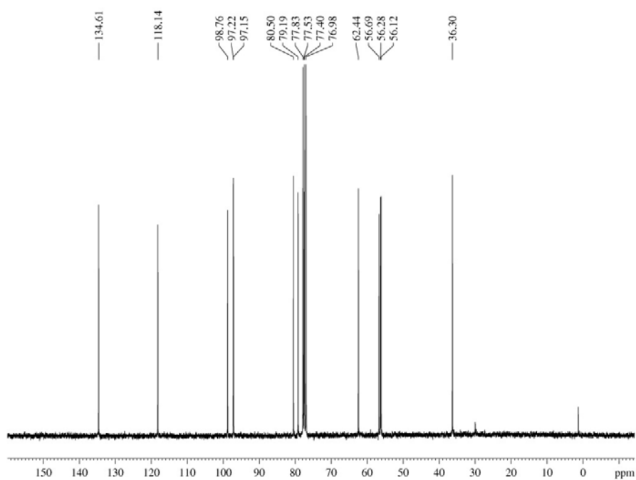
1 H and 13 C spectra of compound 16
