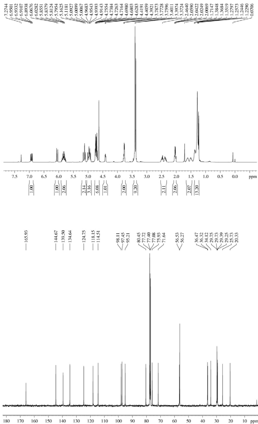
^1\text{H} and ^{13}\text{C} spectra of compound 4
