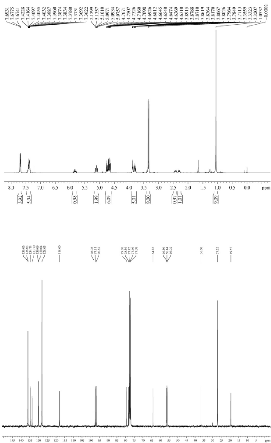
^1\text{H} and ^{13}\text{C} spectra of compound 8
