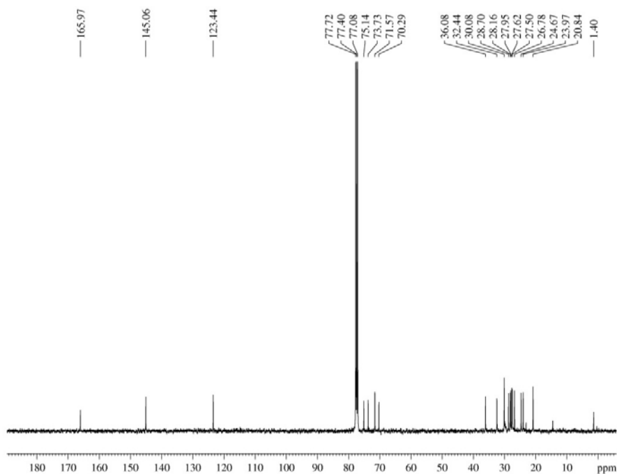
1 H and 13 C spectra of Aspicilin 1
