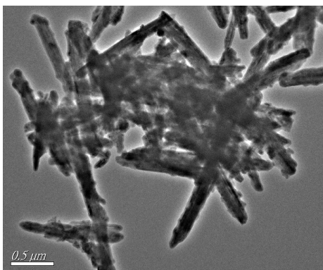
Fig. S1. TEM image of MMINs with the excess amounts of polymerization monomers (0.4 g).
