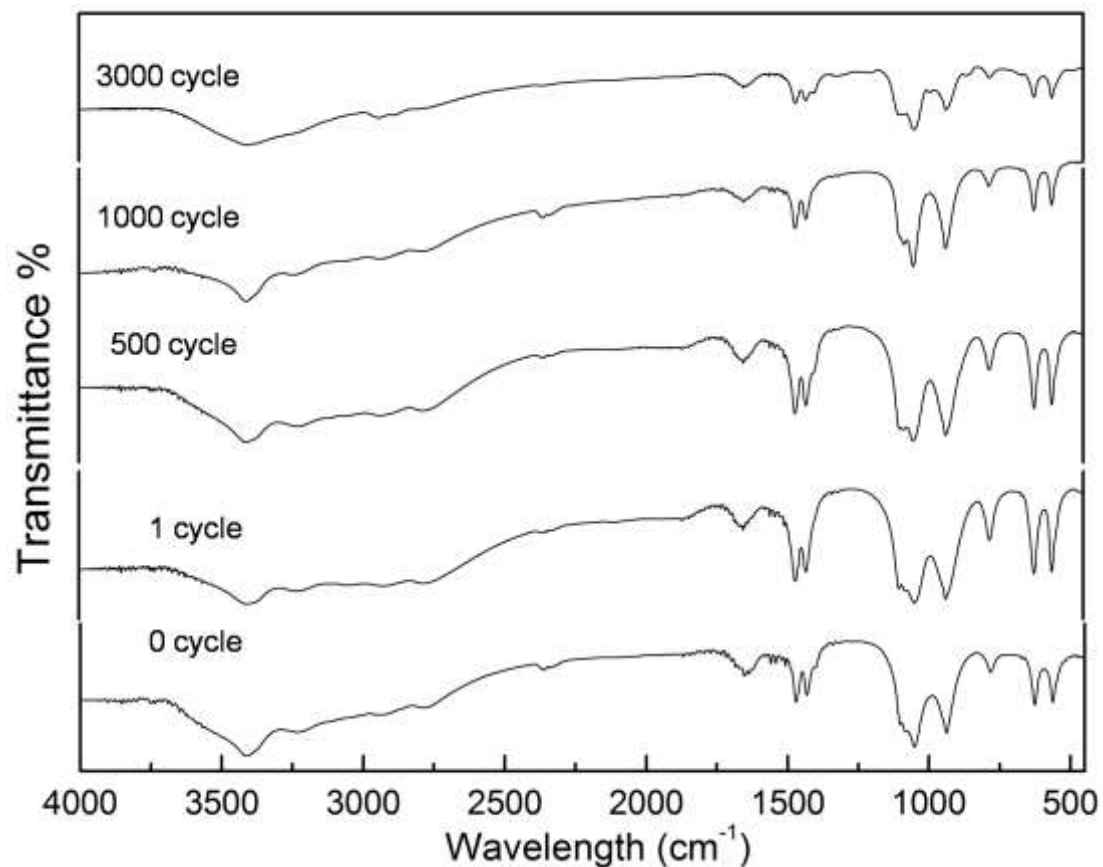
ESI Figure. 2 IR measurements of layered \text{NH}_4\text{CoPO}_4 \cdot \text{H}_2\text{O} microbundles before-0 cycle, and after different charging-discharging cycles-1 cycle, 500 cycle, 1000 cycle, and 3000 cycle.
