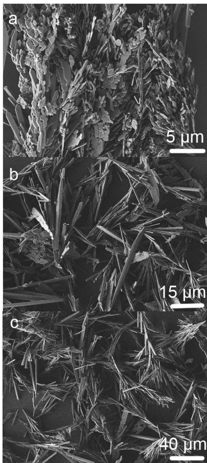
ESI Figure. 1 The product was synthesized under different hydrothermal conditions, (0.10 g of cobalt nitrate and 0.15 g ammonium tertiary phosphate were added into 20.0 mL of distilled water) (a) 8 h; (b) 16 h; and (c) 32 h.
