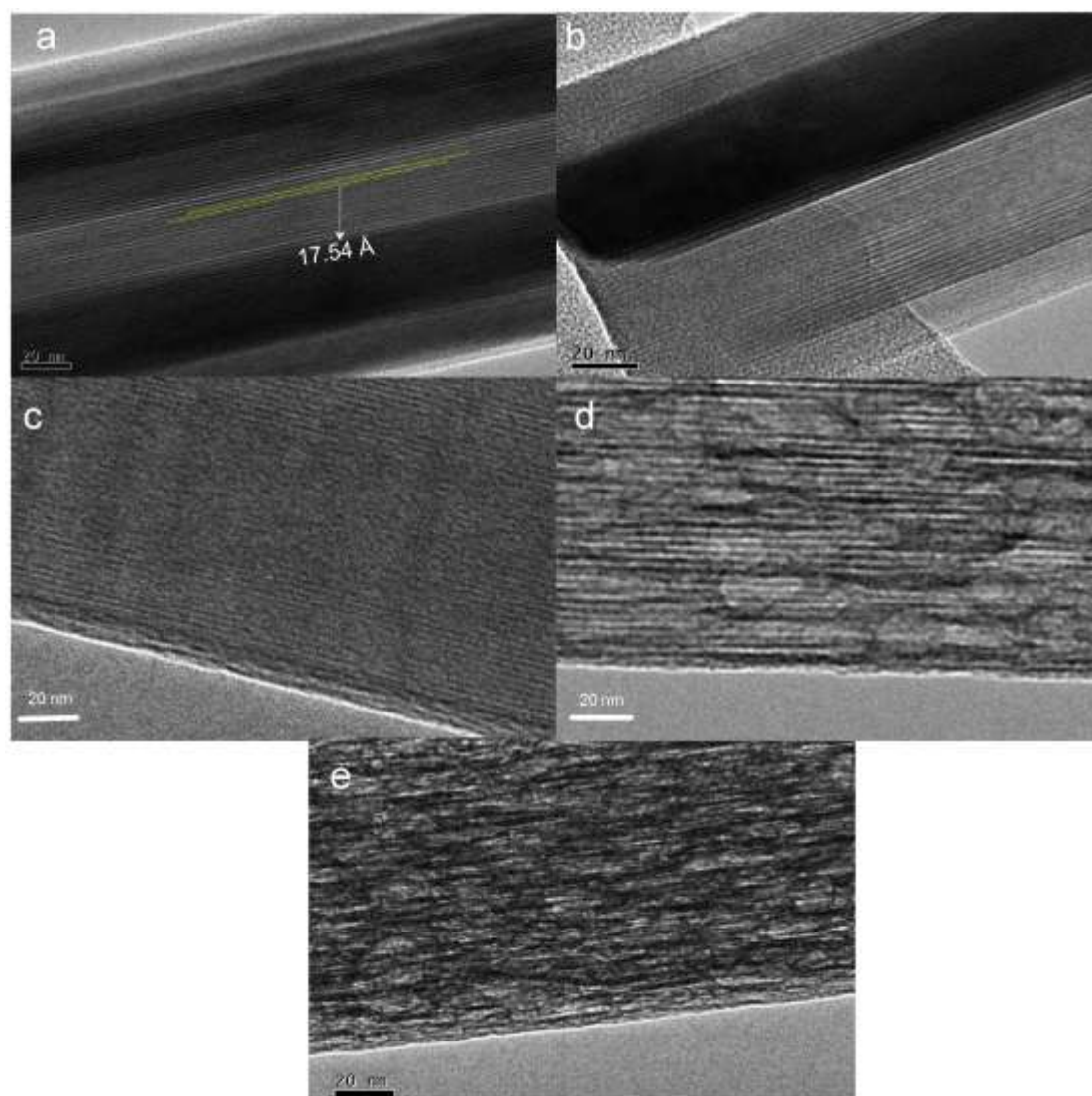
ESI Figure. 3 HRTEM measurements of layered \text{NH}_4\text{CoPO}_4 \cdot \text{H}_2\text{O} microbundles electrodes before (a) 0 cycle, and after different charging-discharging cycles, (b) 1 cycle, (c) 500 cycle, (d) 1000 cycle, and (e) 3000 cycle.
