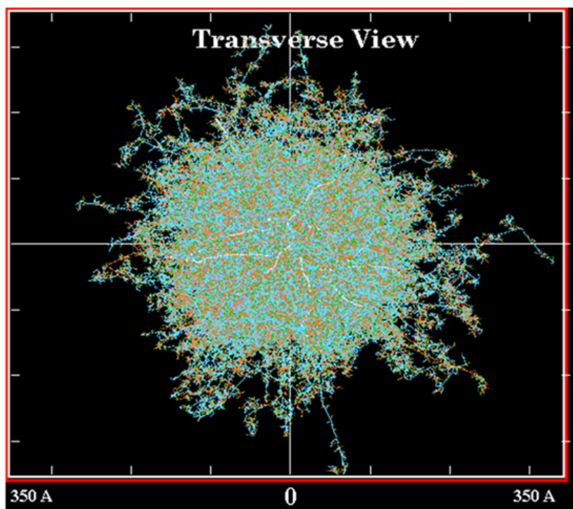
Supplementary figure 1 - SRIM simulation of 1000 Ga ion against \text{Si}_3\text{N}_4 monolayer. The pattern of ion ablation is nearly circular. Due to this the ends of the cut were smooth despite the kerf size being 200nm.
