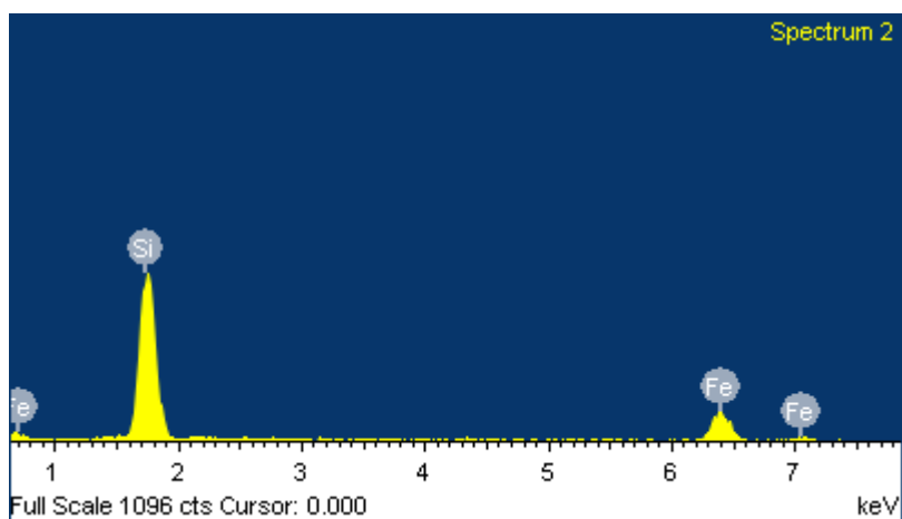
SI 6 EDAX pattern of Fe-SBA-15
