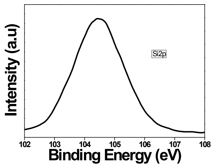
SI 4 XPS spectra of Si2p
