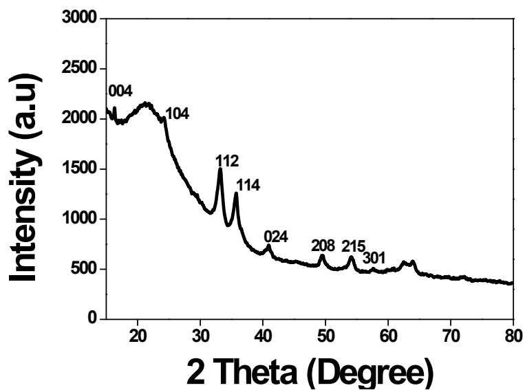
SI 1 Wide angle XRD pattern of Fe-SBA-15
