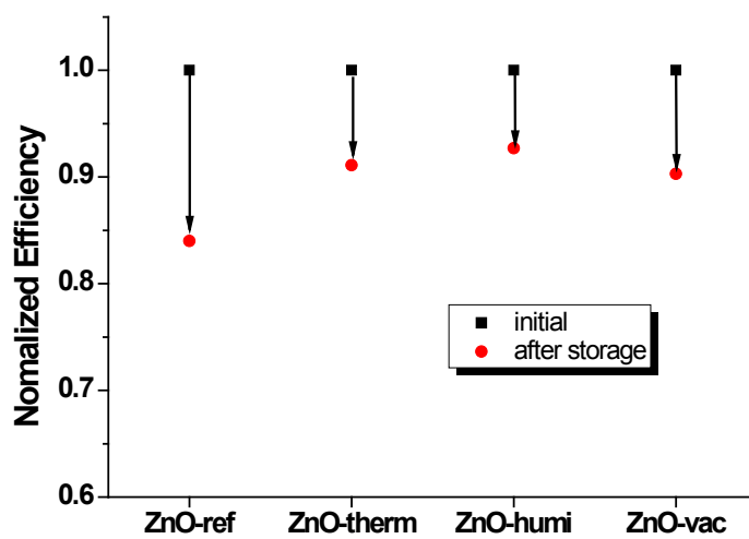
Fig. S1 The stability of the un-encapsulated devices stored in nitrogen-filled glove box for about half a year.
