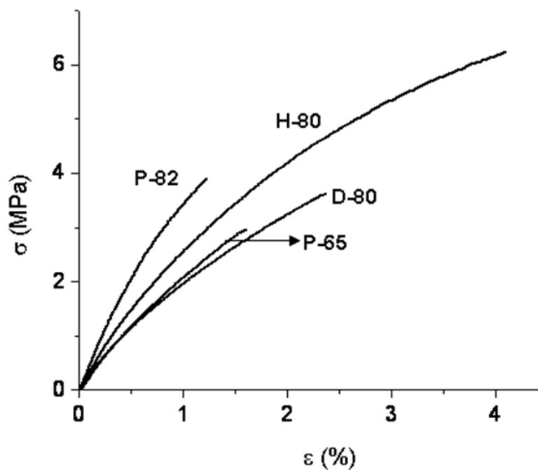
Figure 1S. Stress-strain curves of lactone-DES-MDEA terpolymers
