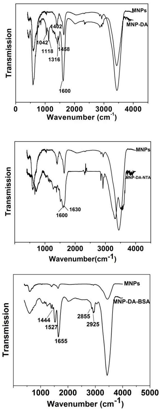
Figure S1. FT-IR spectra of MNPs, MNP-DA, MNP-DA-NTA and MNP-DA-BSA with assignment details.
