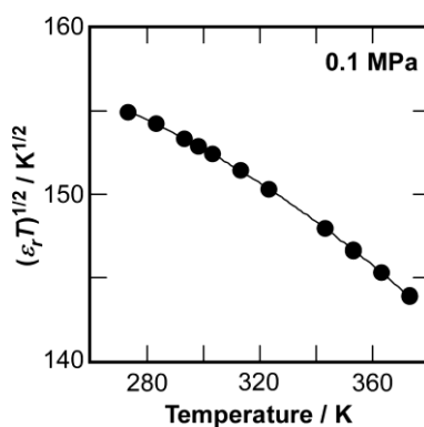
Figure 2S Temperature dependence of (\epsilon_r T)^{1/2} term of water. Static dielectric constants of water at different temperatures are cited from Ref. 20.
