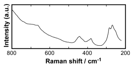
Figure 1S Raman spectrum of solid state TBA + -TiO x prepared by drying the colloidal solution.
