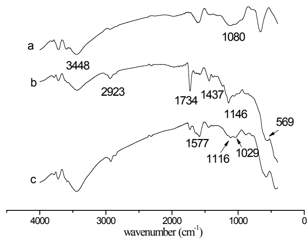
Fig. 2S FT-IR spectra of MWCNTs (a), mag-MWCNTs @PMMA(b), mag-MWCNTs-MIPs (c)
