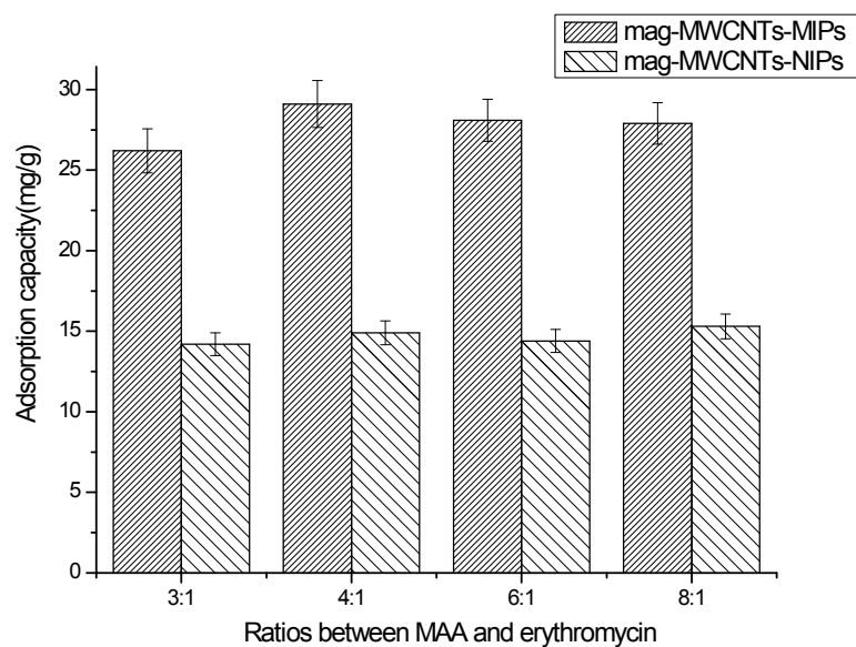
Fig. 1S. Evaluation on the adsorption of mag-MWCNTs-MIPs composited with different ratios between MAA and erythromycin.
