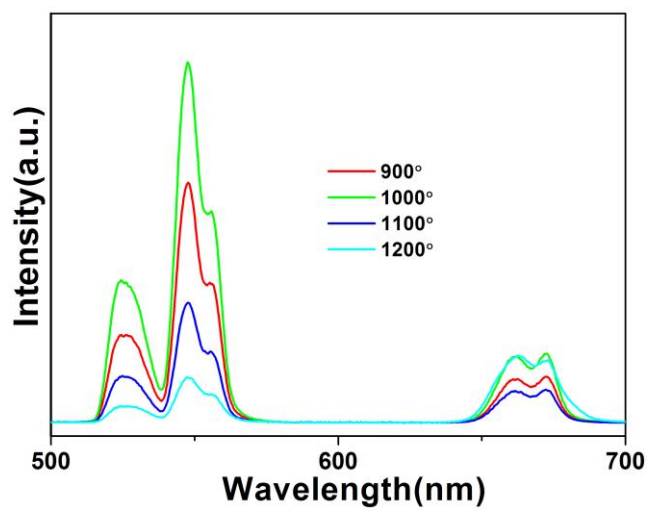
Fig. S1 UC luminescence of \text{CaLa}_{1.93}\text{Yb}_{0.05}\text{Er}_{0.02}\text{ZnO}_5 phosphors annealed at different temperature.
