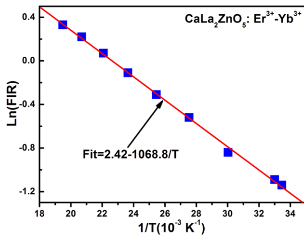
Fig. S2 Monolog plot of the FIR of green upconversion emissions for the {}^2\text{H}_{11/2} , {}^4\text{S}_{3/2} \rightarrow {}^4\text{I}_{15/2} transitions as a function of inverse absolute temperature in the range of 298-513 k.
