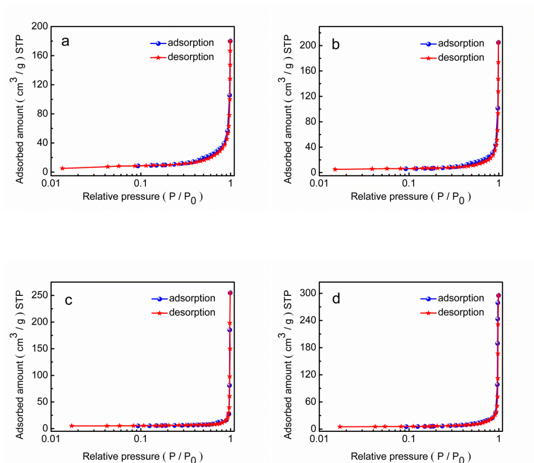
Supplemental Fig. N 2 adsorption/desorption curves of (a) S2, (b) S3, (c) S4 and (d) S6.
