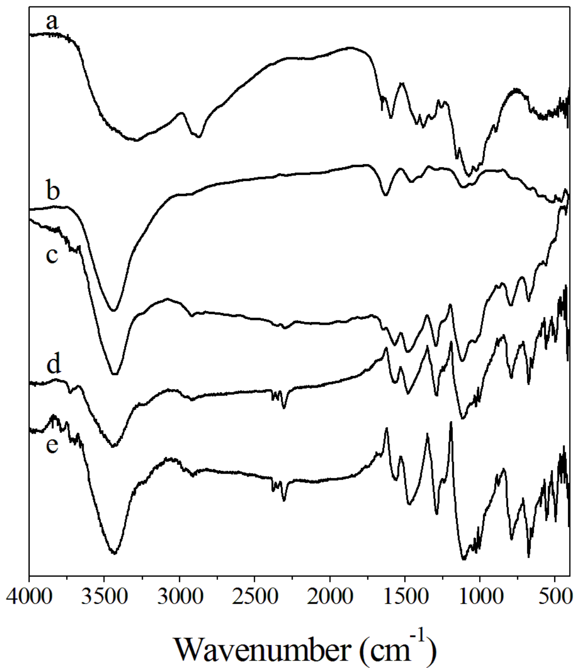
FTIR curves for (a) chitosan, (b) PANi-chitosan 40/60 wt/wt, (c) PANi-chitosan 50/50 wt/wt, (d) PANi-chitosan 66.7/33.3 wt/wt and (e) PANi.
