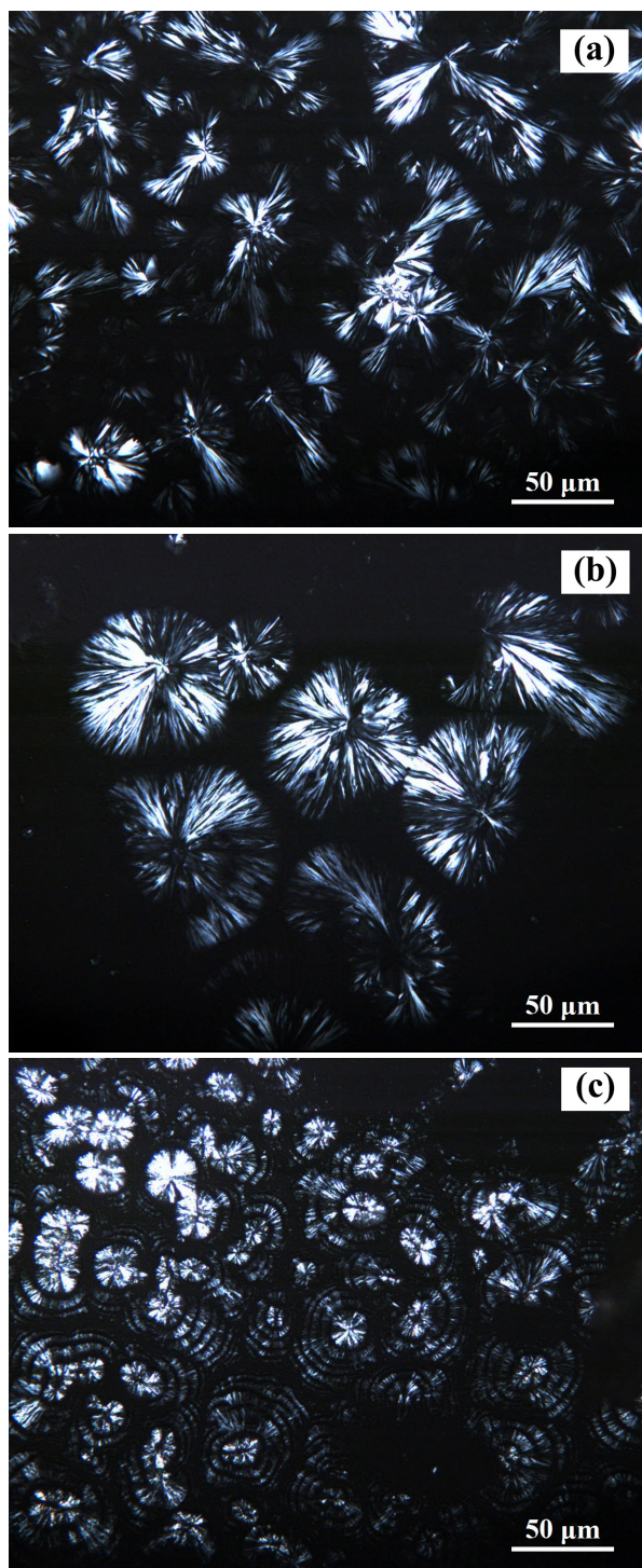
Figure S2. PCL samples were treated with CO 2 at 28 °C for 4 h at various pressures: (a) 1 MPa; (b) 2 MPa; (c) 8 MPa.
