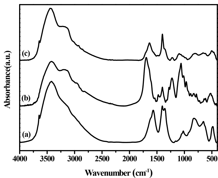
Figure S1. FT-IR spectrum of (a) Ni-In-CH 3 COO - LDHs, (b) DNA, (c) DNA-LDHs complexes.
