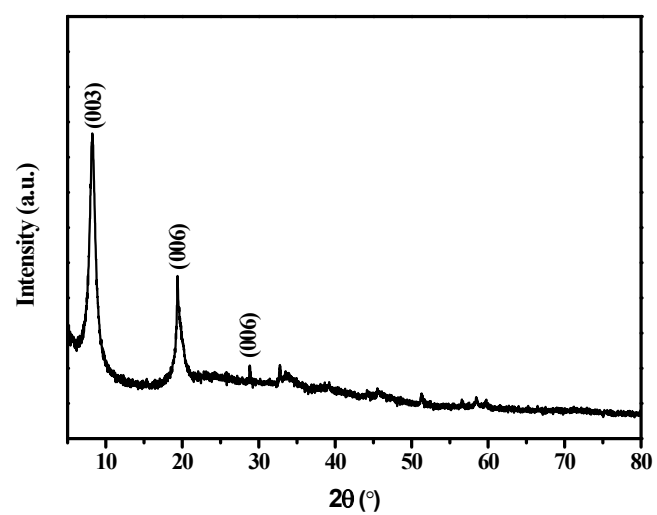
Figure S4. XRD pattern of Ni-In LDHs after DNA desorption by the addition of \text{HPO}_4^{2-} .
