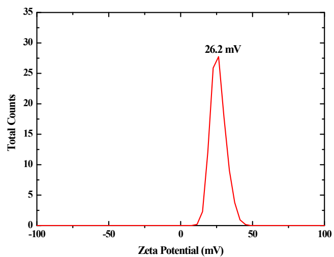
Figure S3. Zeta potential curve of the colloidal suspension of Ni-In ELDHs nanosheets.
