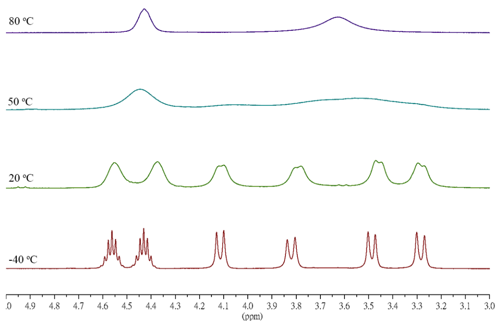
Fig. S2. Variable temperature dependent ^1\text{H} NMR spectra of 6 (*: grease; **: Hex) ranging from 3.0-5.0 ppm.
