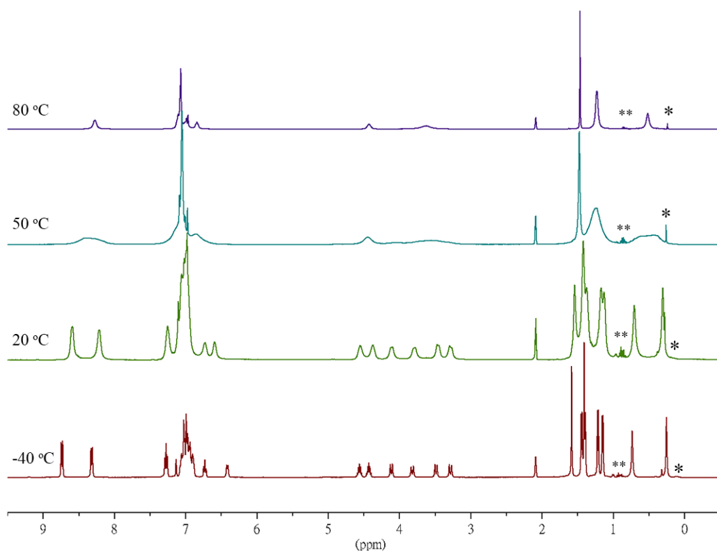
Fig. S1. Variable temperature dependent ^1\text{H} NMR spectra of 6 (*: grease; **: Hex).
