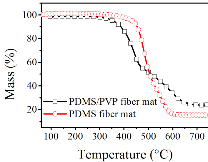
Fig. S1 TGA curves of PDMS/PVP and PDMS fibers.
