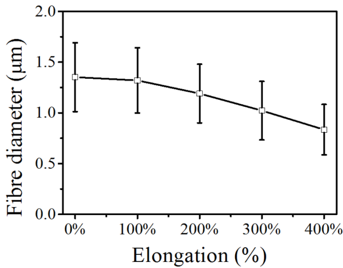
Fig. S2 Influence of elongation ratio on PDMS fiber diameter.
