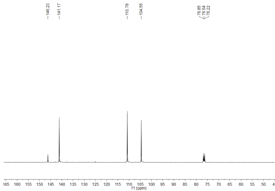
Figure S2 13 C NMR spectra of 2Fu
