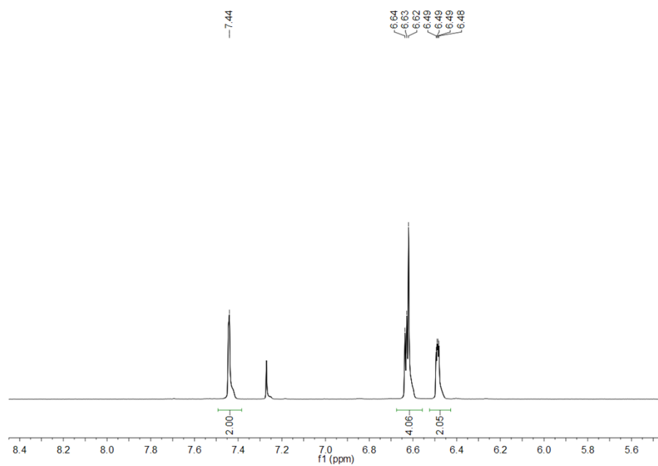
Figure S3 1 H NMR spectra of 3Fu
