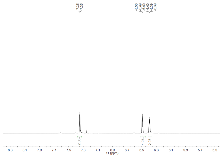
Figure S1 1 H NMR spectra of 2Fu
