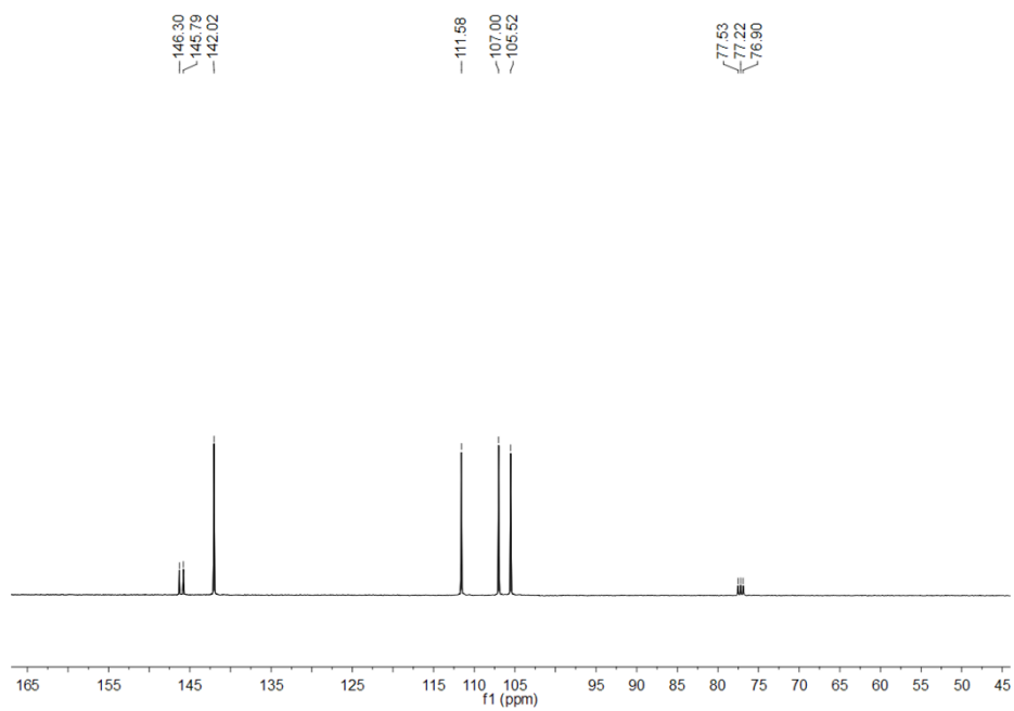
Figure S4 ^{13}\text{C} NMR spectra of 3Fu
