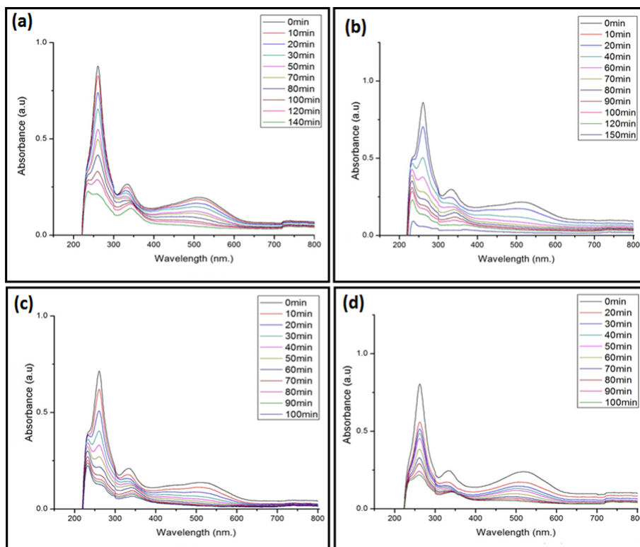
SI 1: Spectral changes during UV-catalytic degradation for BiOI at (a) x=1%, (b) x=2%, (c) x=3% and (d) x=4% (w/v).
