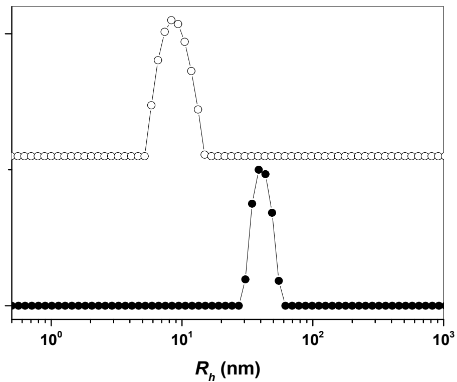
Fig. S2 Size distribution function of silica particles by DLS: ○ 30R12, ● 30R50
