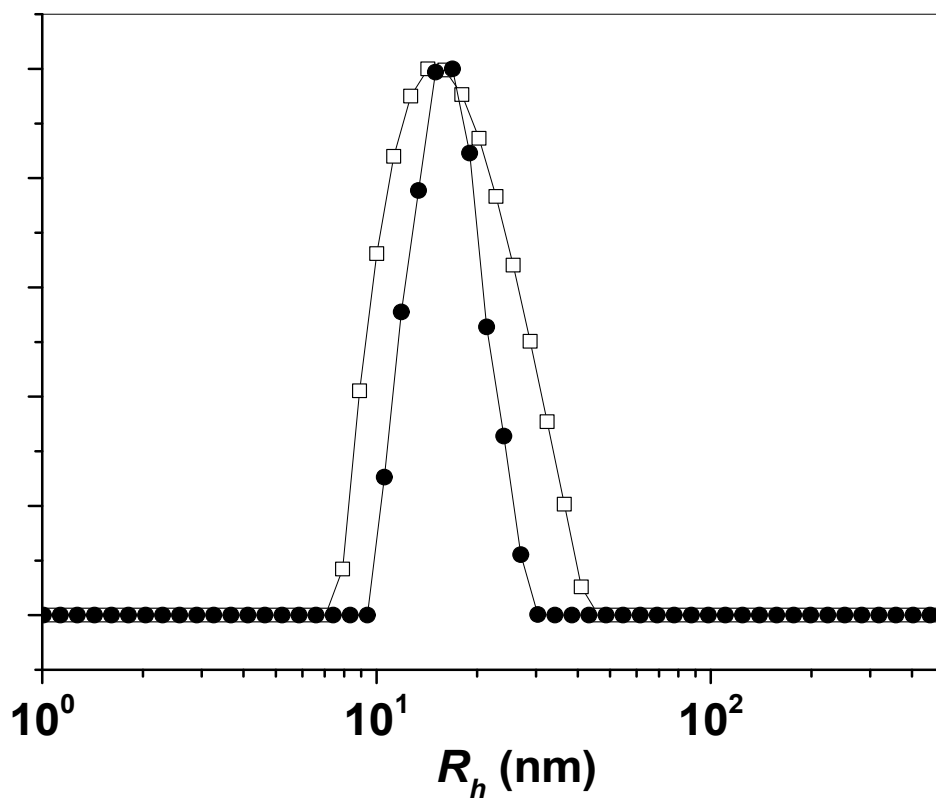
Fig. S1 Size distribution function of silica particles by DLS: ●TM40, □BINDZIL2040.
