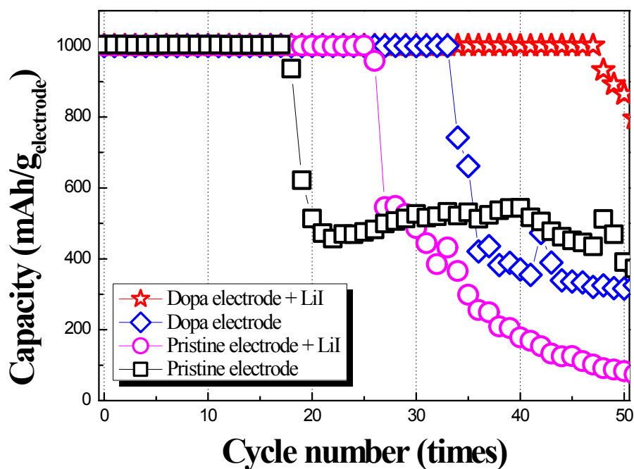
Figure S1 : Cyclic performance of the pristine and dopa electrodes at a current density of 1000 mA·g -1 , measured using plain and LiI-containing electrolytes.
