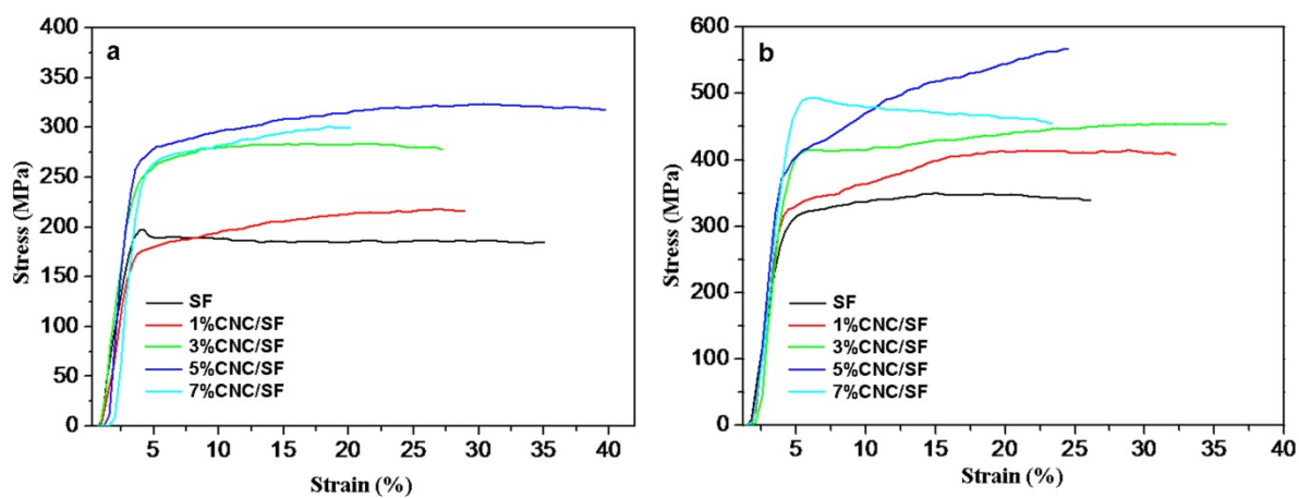
Fig. S3. Stress-strain curves of regenerated SF fibers and various CNC/SF fibers with 1X (a) and 2X (b) of post draw.
