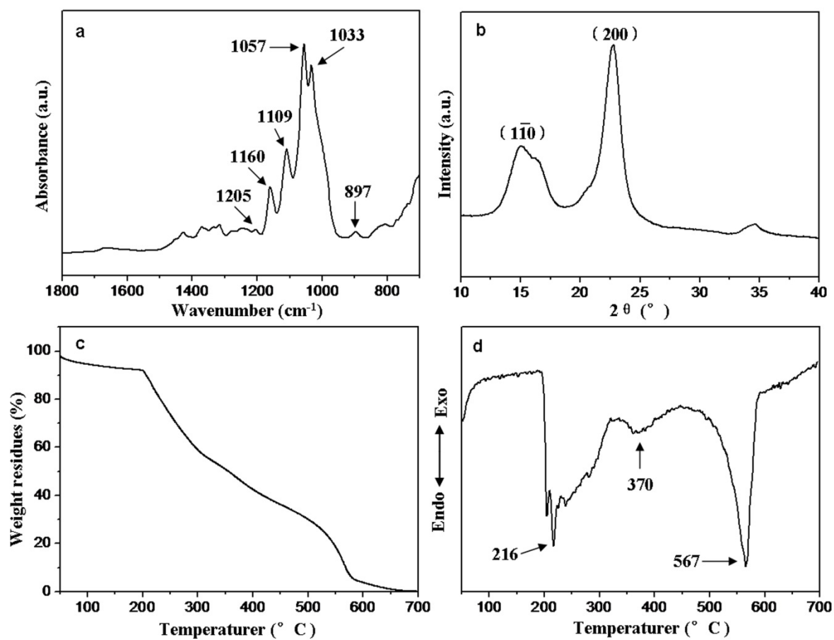
Fig. S2. FTIR spectra (a), XRD patterns (b), TGA (c) and DTG (d) curves of CNC.
