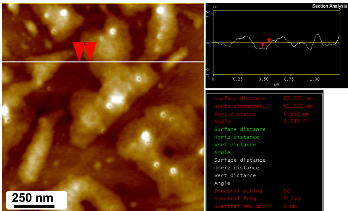
Fig. S1: AFM height image of PE-HRG with the corresponding line profile at the edge.
