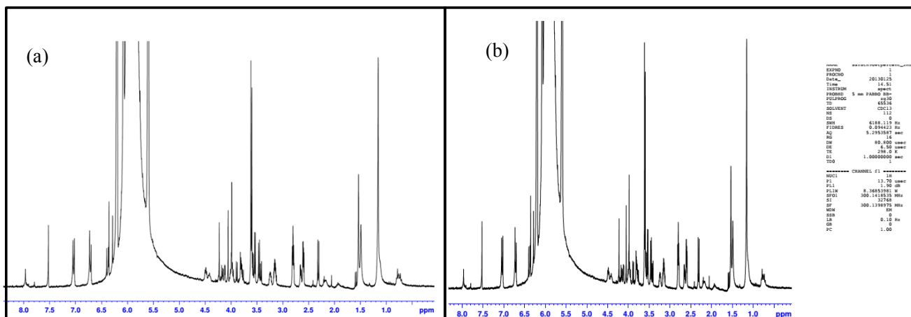
Figure 1: Results of the NMR experiment for 90 % w/w blend using 1,1,2,2, tetrachloro ethane as solvent. The solution was made by mixing at 150 °C for 20 min
