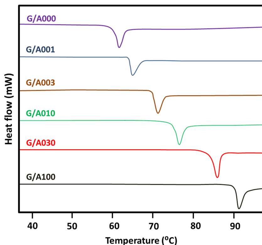
Fig. S1 Typical DSC thermograms of various AM samples.
