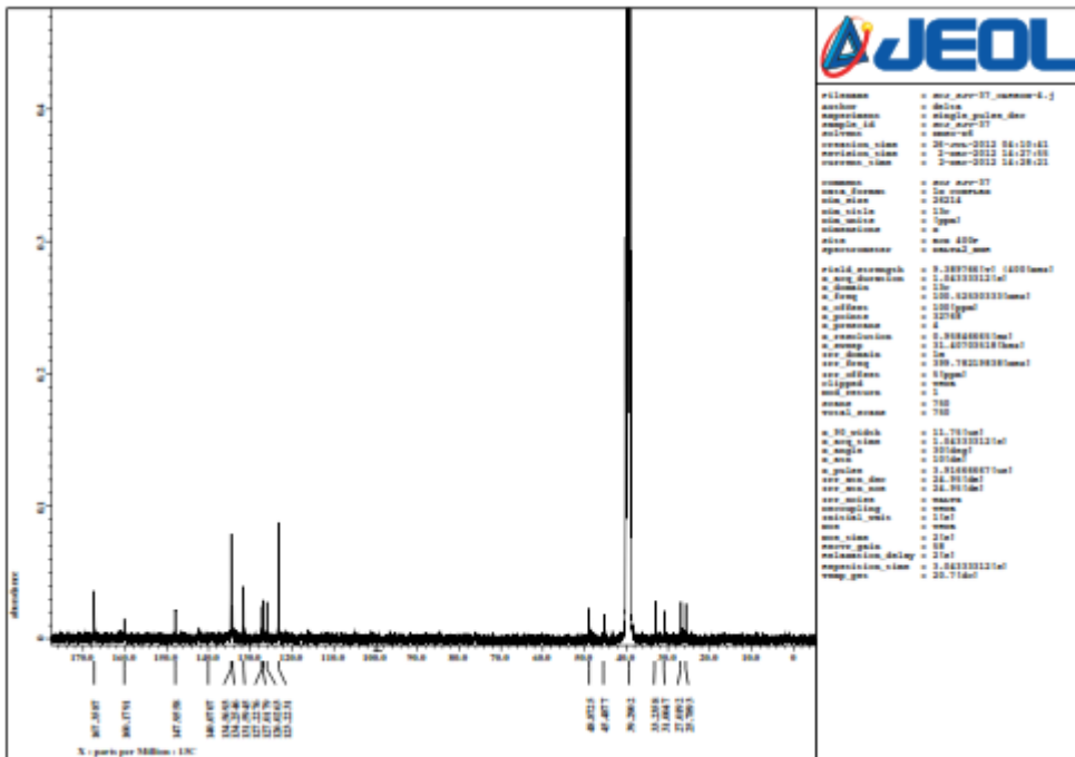
4-(4-(4-(Indolin-2,3-dion-1-ylmethyl)-1H-1,2,3-triazol-1-yl)butyloxy)quinazoline (1i)
