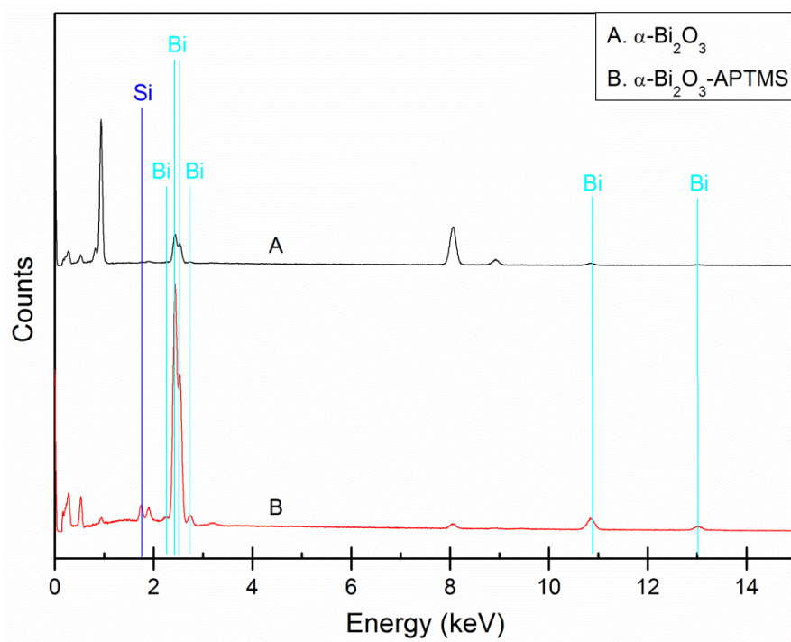
Fig. S1: EDS spectra of (A) uncoated \alpha\text{-Bi}_2\text{O}_3 NPs and (B) APTMS coated \alpha\text{-Bi}_2\text{O}_3 NPs.
