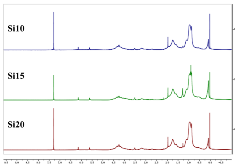
Fig. S2 The ^1\text{H} NMR of the nanogels.
