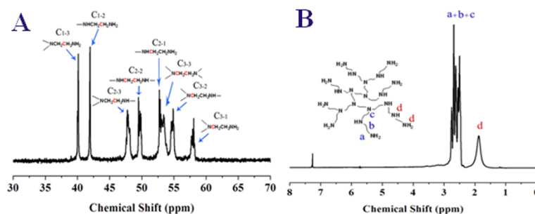
Figure S1. (A, B) 13 CNMR and 1 HNMR spectra of HPEI in CDCl 3
