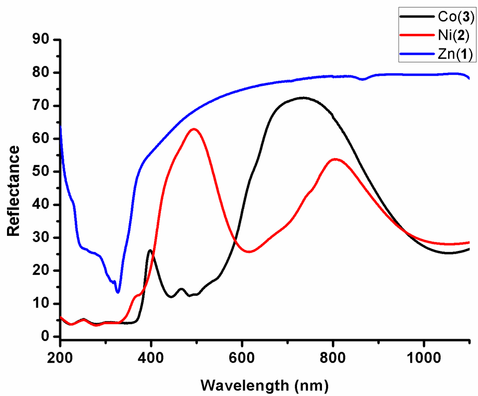
Figure S5: Solid state diffuse reflectance spectra of 1-3.
