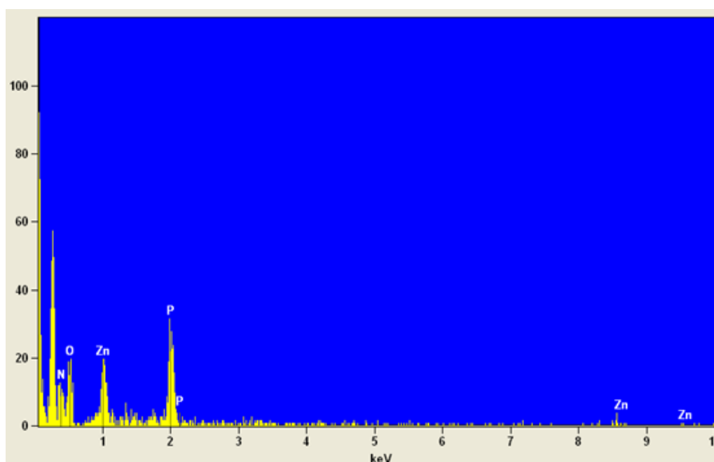
Figure S1: EDX spectrum of 1.
