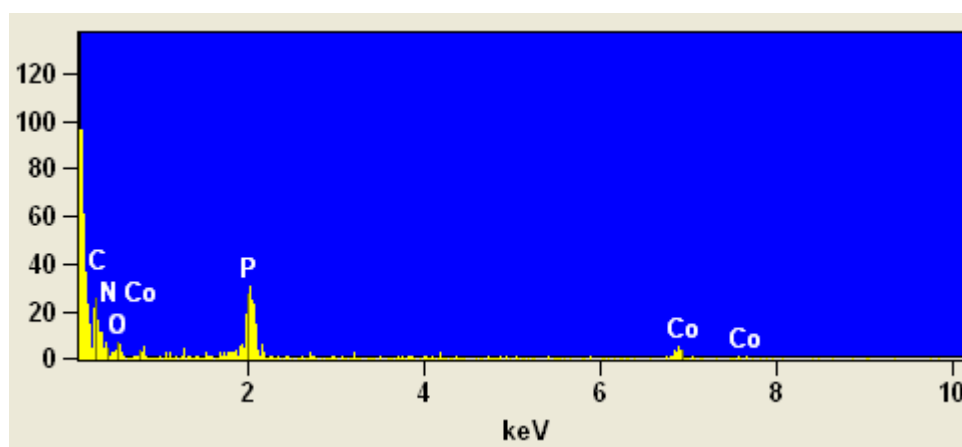
Figure S2:EDX spectrum of 2.
