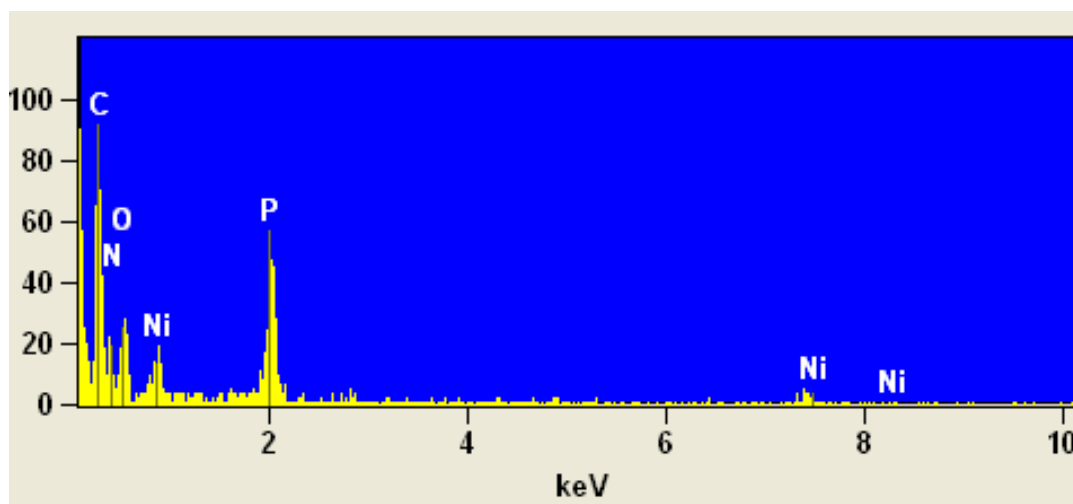
Figure S2:EDX spectrum of 2.
