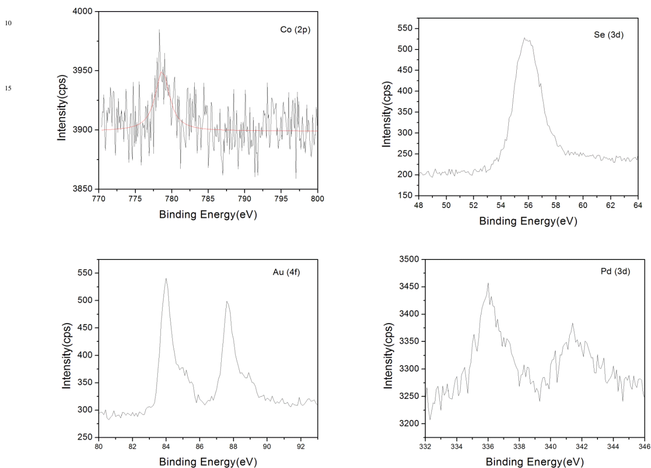
Fig. S1: The XPS spectra collected from the Au 3 Pd-CoSe composite nanoparticles after sputtering for 10 s.
