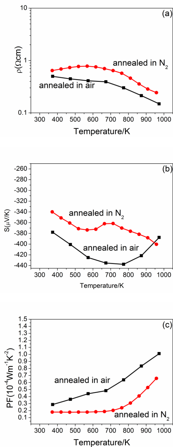
Fig.S1 Electrical properties measurements on \text{In}_{2-2x}\text{Lu}_{2x}\text{O}_3 ( x=0.05 ) between 373K and 973K: Electrical resistivity(a) Thermopower(b) and Power factor(c). Samples were annealed in air and \text{N}_2 respectively before measurements
