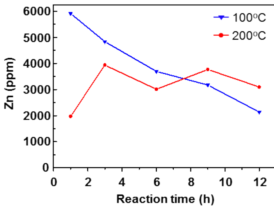
Figure S2. ICP-AES analyses of the variation of supernatant Zn concentration, after reaction at 100 and 200 °C for different reaction times.
