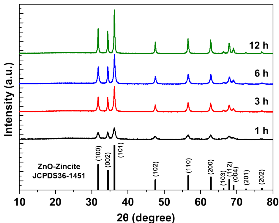
Figure S1. XRD patterns of ZnO particles prepared at 150 °C for different reaction times.
