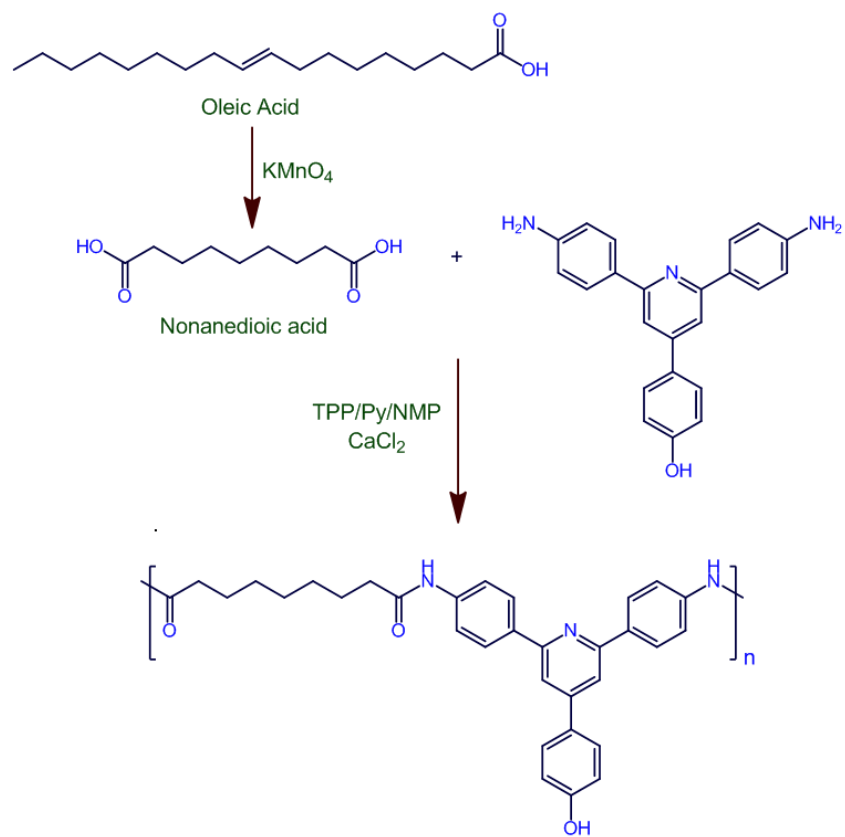
Scheme S2. Polycondensation reaction of the diacid derived from oleic acid with the diamine
