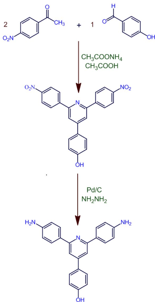
Scheme S1. Synthesis of the diamine
