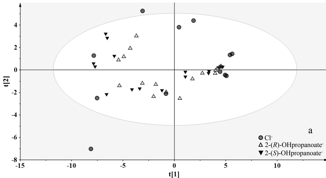
S10: PCA Scores Plot in the Bacteria and Fungi toxicity model for imidazolium-based ILs. S10a: anions distribution; S10b: side chains distribution. Imidazolium side chains labels in S11.
