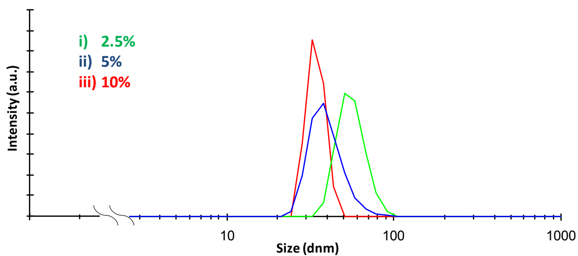
Figure S4. DLS curves of the synthesized FAU nanocrystals after sonication.
