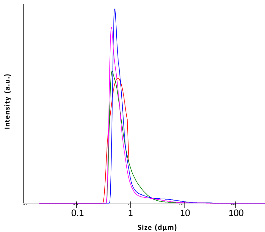
Figure S5. DLS curves of micron-sized FAU crystals collected before sonication (red line) and after 10 (green line), 20 (pink line) and 30 (blue line) minutes of sonication.
