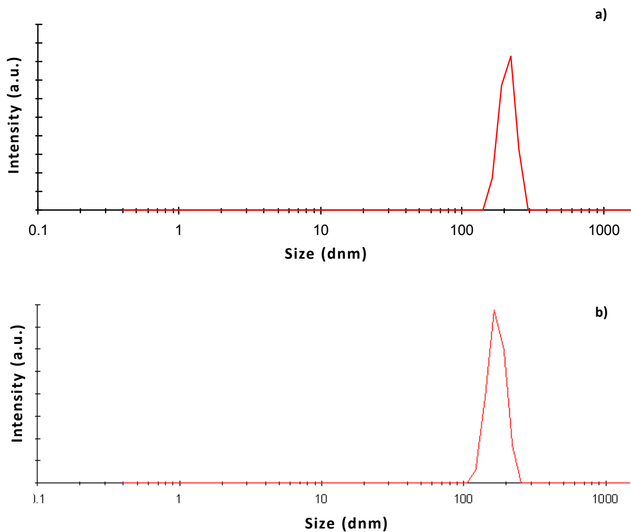
Figure S2. DLS curves before(a) and after (b) sonication of the synthesized FAU nanocrystals obtained after 36h of reaction without using the seeded support.
