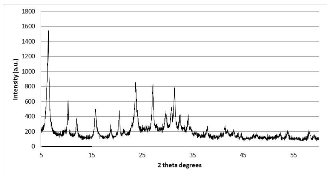
Figure S3. XRD pattern collected on micron-sized FAU zeolites.
