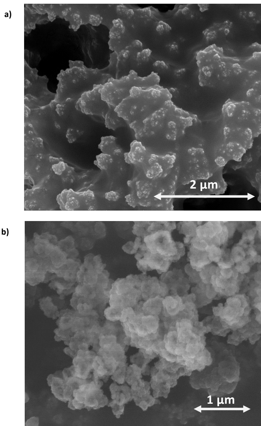
Figure S1. SEM image of the amorphous phase (a) and crystalline product (b) obtained after 36h of reaction without using the seeded support.
