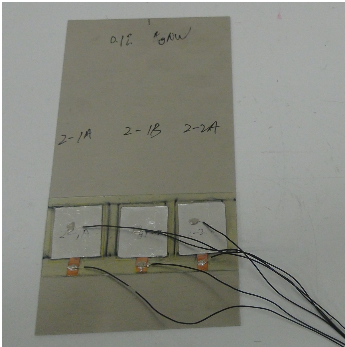
ESI-3 Attachment of piezofilms on Al plate
