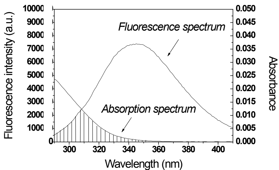
Fig. S1. Spectral overlap of nalorphine absorption with fluorescence of HSA-nalorphine complex. Concentrations of HSA and nalorphine were all 1 \times 10^{-6} M.
