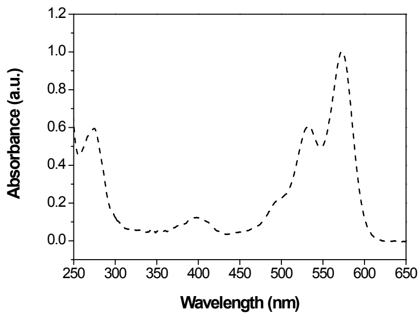
Fig. S4 UV-vis absorption spectrum of compound 7 in \text{CHCl}_3 at room temperature.
