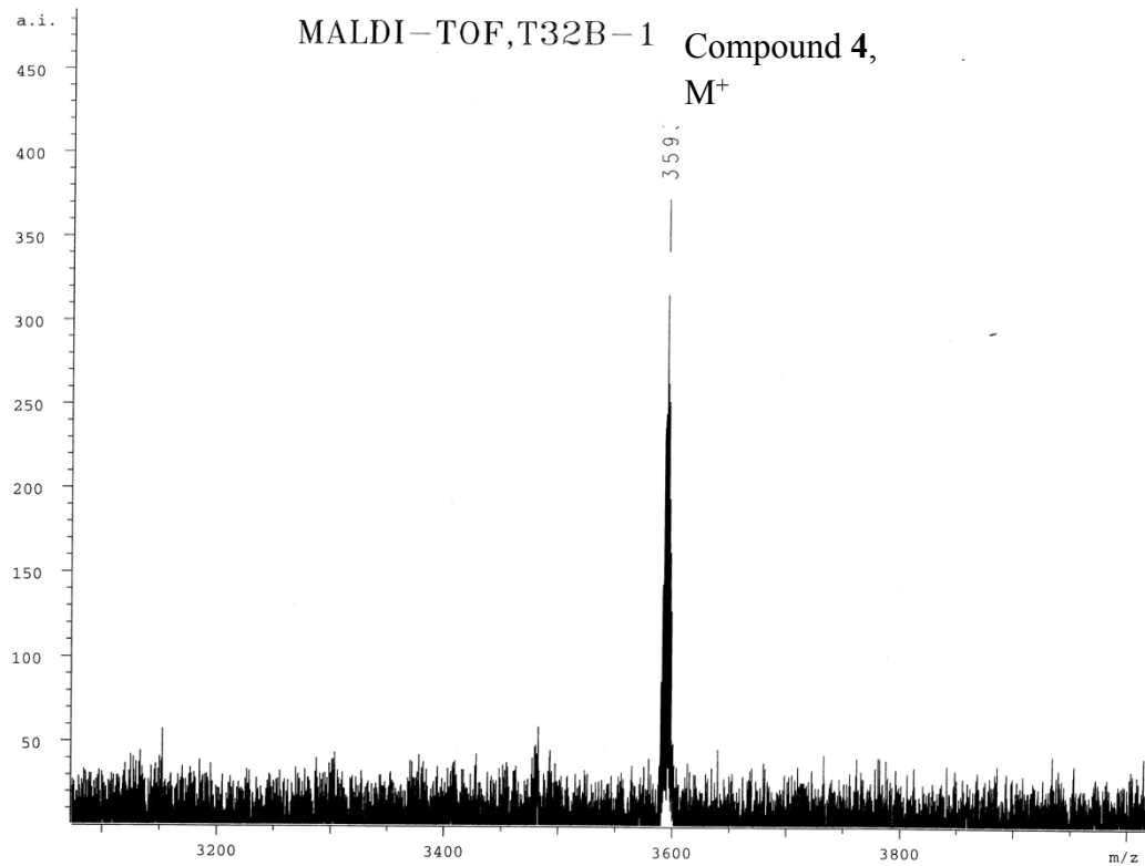
Fig. S1 MALDI-TOF MS spectra of compound 4
