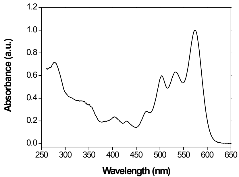
Fig. S5 UV/Vis absorption spectrum of compound 8 in \text{CHCl}_3 at room temperature.
