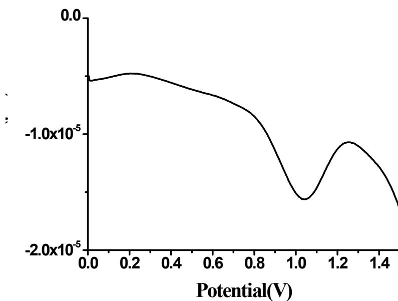
Fig. S1 DPV curve of 1 mM melamine in 0.1 M phosphate buffer (pH 10) at CCG modified GC electrode, Scan rate: 25 mV/s.
