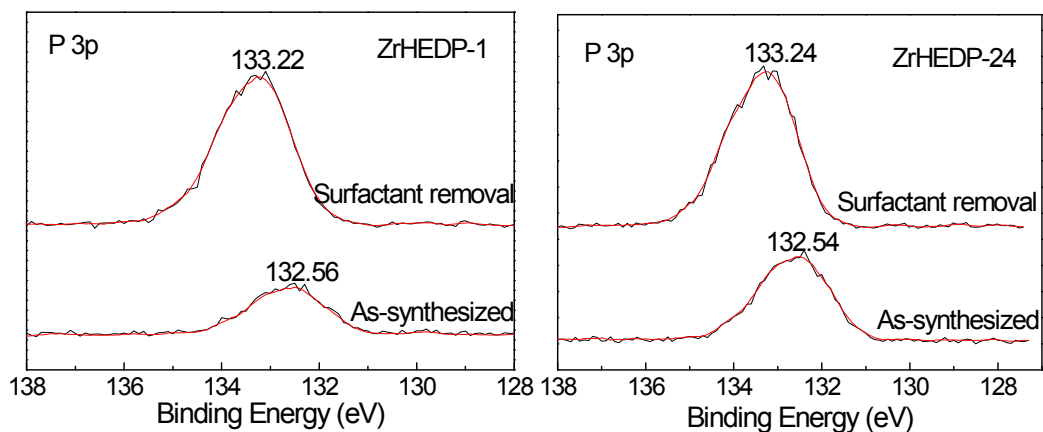
Fig. S3 XPS P 3p spectra for ZrHEDP-1 (left) and ZrHEDP-24 (right), before and after surfactant removal.
