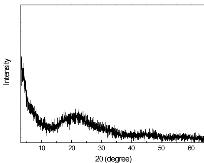
Fig. S1 Wide-angle powder X-ray diffraction pattern of surfactant-removed ZrHEDP- x .
