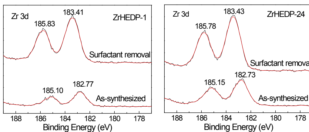
Fig. S2 XPS Zr 3d spectra of ZrHEDP-1 (left) and ZrHEDP-24 (right), before and after surfactant removal.
