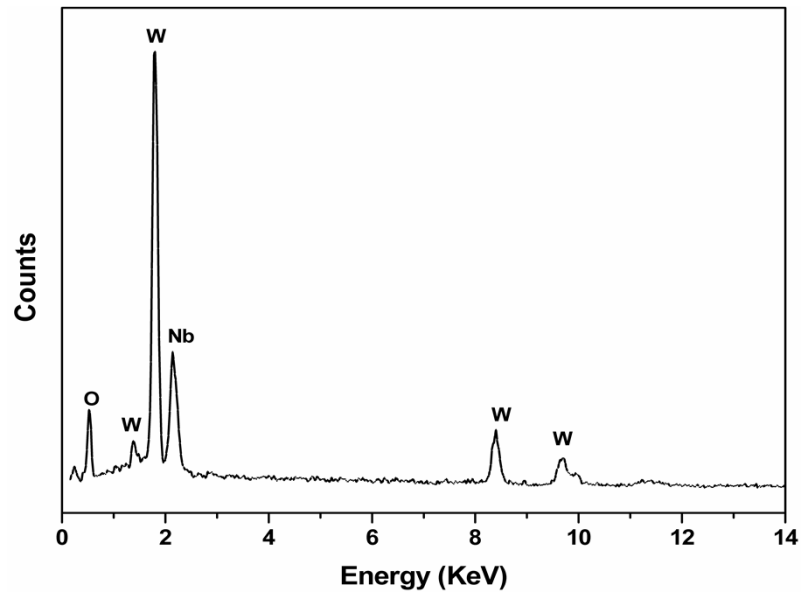
Fig.1. EDX spectra of Nb-doped \text{WO}_3 (the atomic ratio of Nb/W is 0.03)
