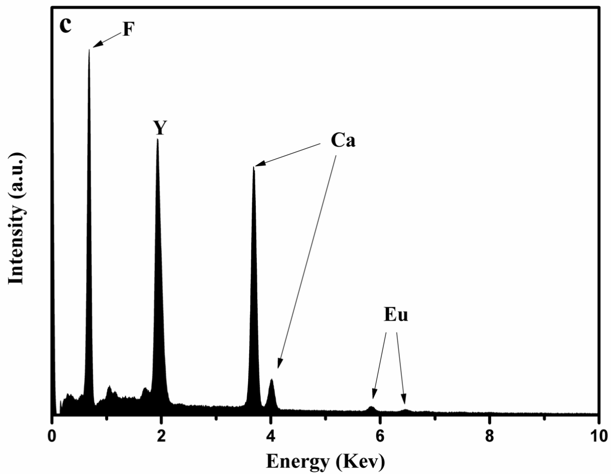
Figure S2 The EDX spectrum of Eu-doped \text{CaF}_2\text{-YF}_3 .
