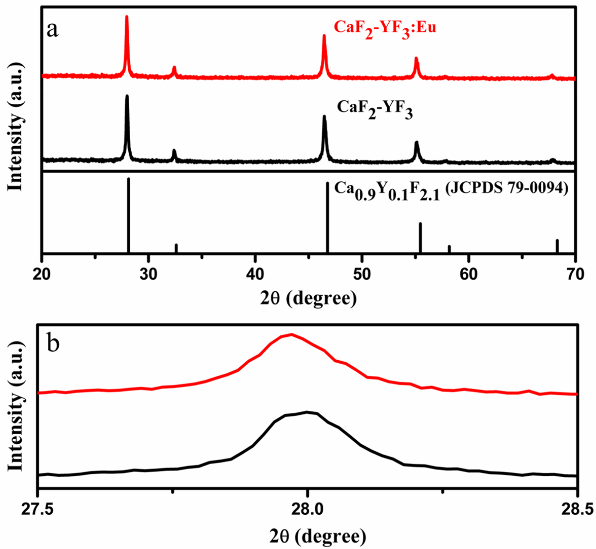
Figure S1 (a) The XRD patterns of \text{CaF}_2\text{-YF}_3 (black line) and Eu-doped \text{CaF}_2\text{-YF}_3 (red line), and (b) their corresponding partial enlarged detail.
