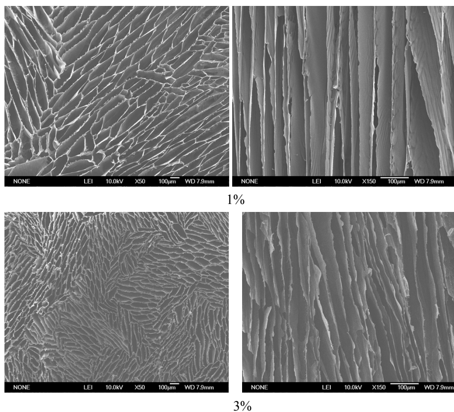
Fig. S1. SEM photos of cross sections (left) and vertical sections (right) of Gel foams with different Gel concentrations (1%, 3%)
