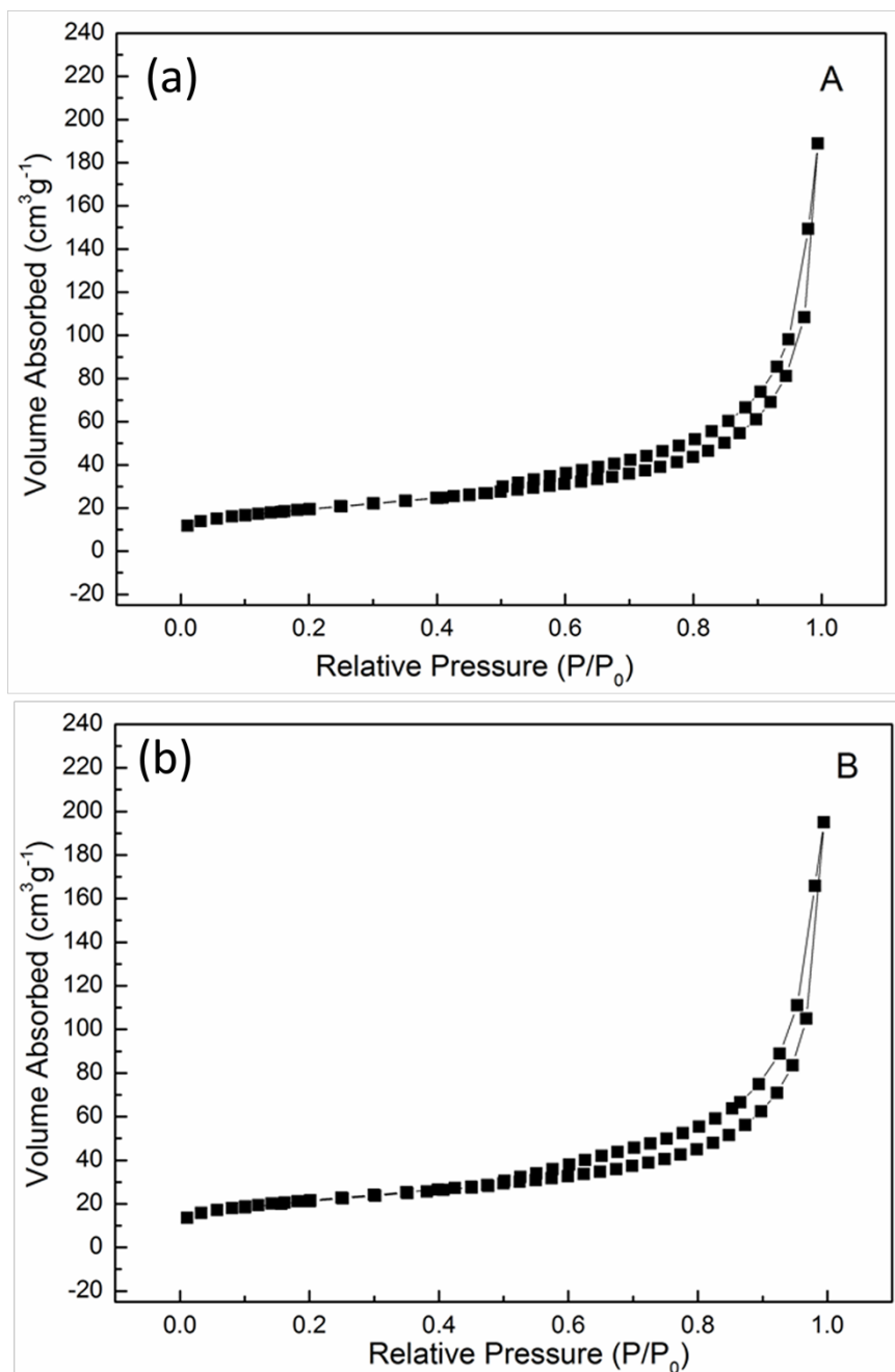
Figure S2. N 2 adsorption–desorption isotherm of (a) A and (b) B samples.
