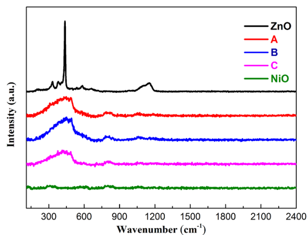
Figure S1. Raman spectra for ZnO, NiO, A, B and C samples.
