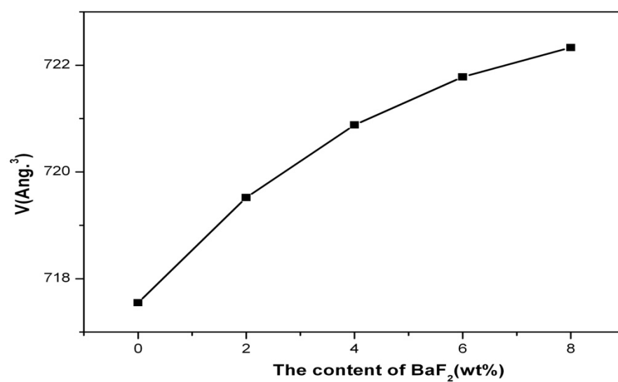
Fig.S1 Unit cell volume dependences on the concentration of \text{BaF}_2
