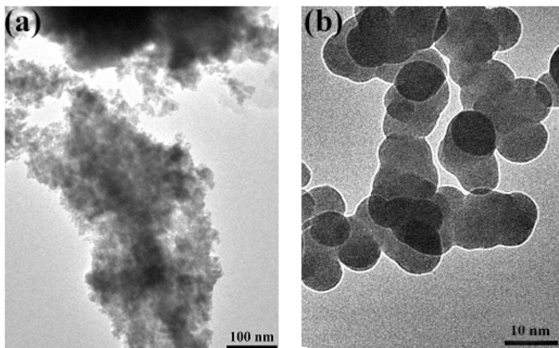
Fig. S1. TEM images of NiO nanoparticles prepared by thermal decomposition of nickel oxalate nanofibers.
