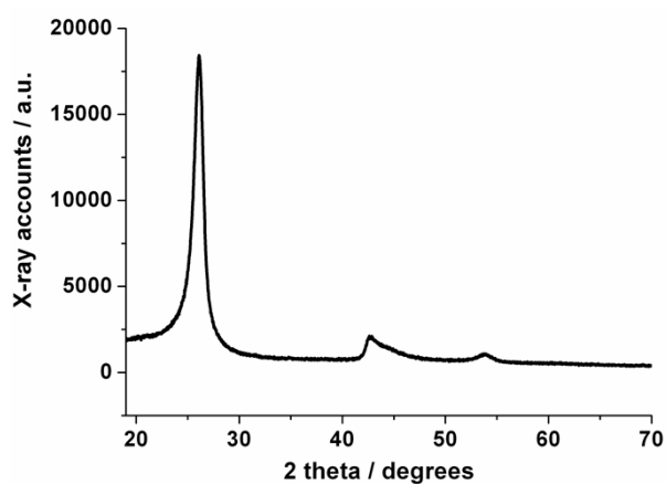
Figure S1. XRD pattern of ionothermal carbon after acid etching.
