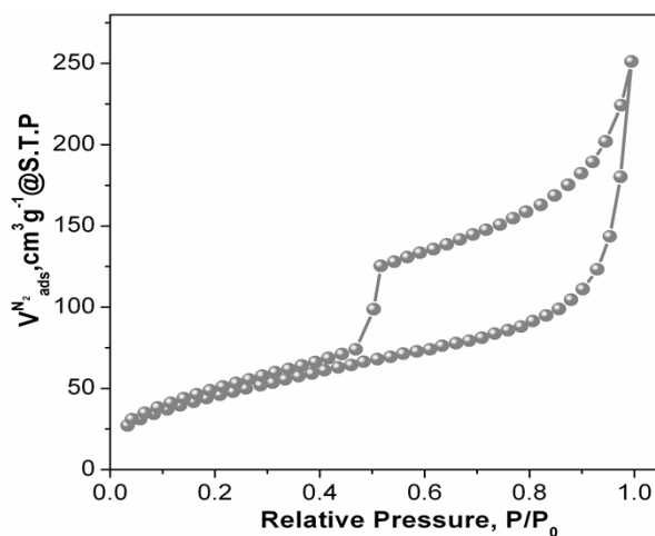
Figure S3. N 2 sorption of ionothermal carbon after acid treatment.
