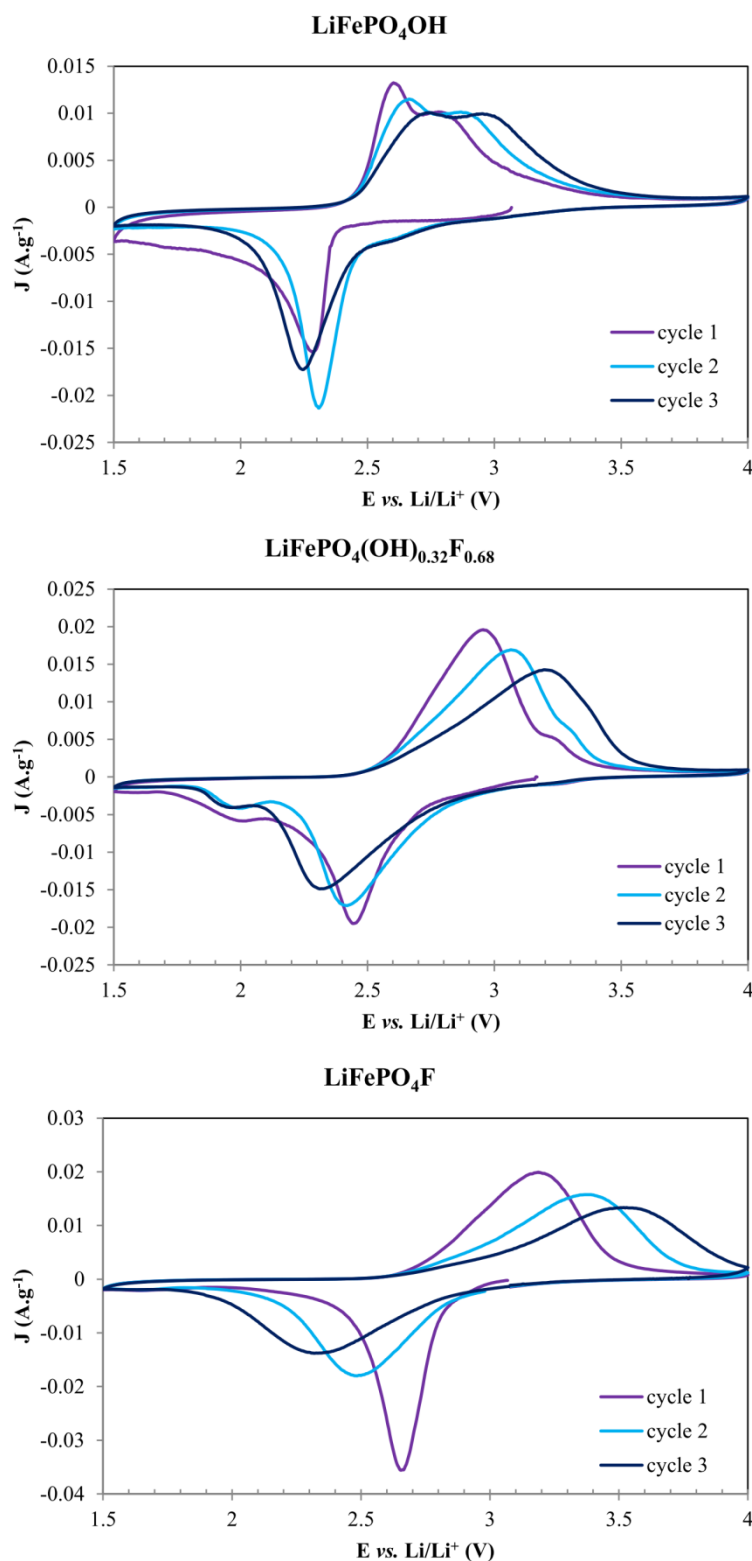
Figure S1. First 3 cycles of CV for the three iron tavorite phases.
