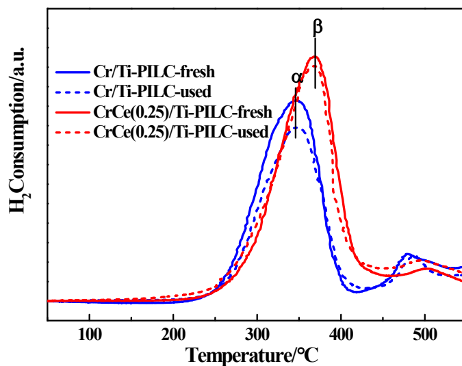
Fig. S2. H 2 -TPR of fresh and used samples: Cr/Ti-PILC and CrCe(0.25)/Ti-PILC.
