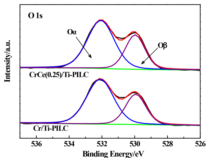
Fig. S1 XPS spectra of O 1s in the Cr/Ti-PILC and CrCe(0.25)/Ti-PILC catalysts
